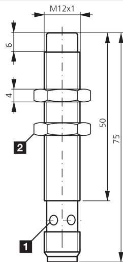
1) LED 4 x 90° (gelb) / LED 4 x 90° (yellow) / LED 4 x 90° (jaune) de clé 17 mm 2) Schlüsselweite 17 mm / Width over flats 17 mm / Ouverture de clé 17 mm
