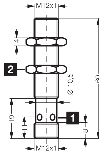
1) LED 4 x 90° (gelb) / LED 4 x 90° (yellow) / LED 4 x 90° (jaune) de clé 17 mm 2) Schlüsselweite 17 mm / Width over flats 17 mm / Ouverture de clé 17 mm
