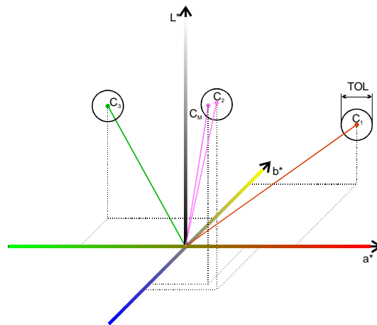
Fig. 5: Diagram for explaining the recognition mode “Check Spere”
