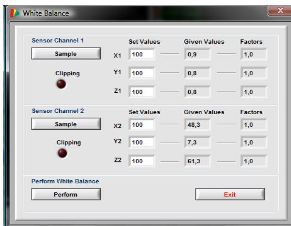
Fig. 10: White balance window
