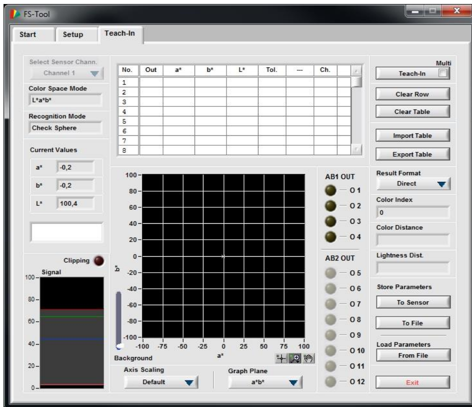
Fig. 11: Teach-In window for teaching colors and displaying recognition results
