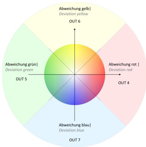
Fig. 12 Output Coding in Deviation Mode for the Tolerance Parameter ab on the outputs OUT4 – OUT7
