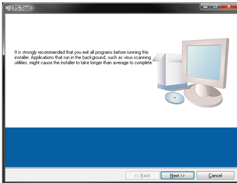
Fig. 1 Installer window
