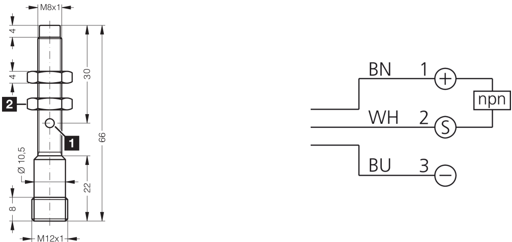
1) LED 2) Width over flats 13 mm BN: brown BU: blue WH: white
