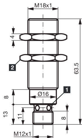
1) LED 2) Width over flats 24 mm BN: brown BU: blue WH: white
